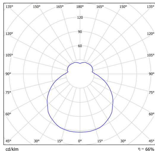
cd/klm — C0 - C180 — C90 - C270 \eta = 66\%
