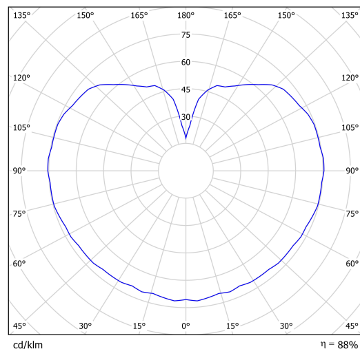
cd/klm — C0 - C180 — C90 - C270 \eta = 88\%
